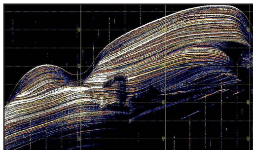
Angola Basin, dense sediment layering recorded by METEOR 2008 (450 m water depth, 50 m penetration)
