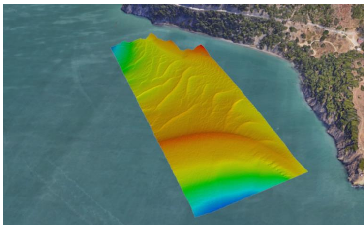
WAM-V 16 ASV hydrographic survey results
